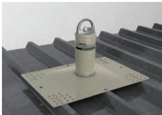
Metal Sheathing
